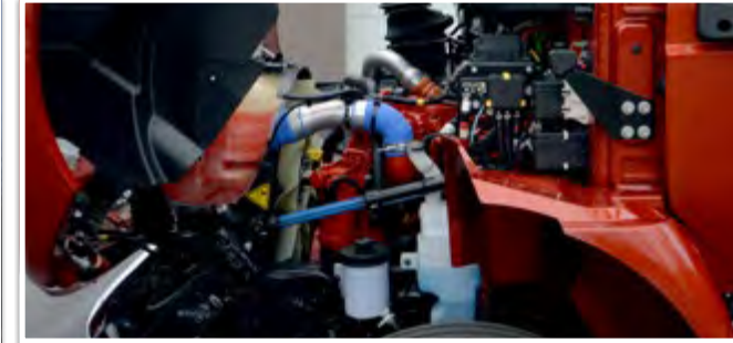
Key fluid reservoirs are translucent for quick inspection and many of the caps are tethered, saving time and frustration from dropped or lost caps
